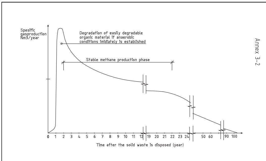
Figure 4 Schematic presentation of the degradation process at landfills
