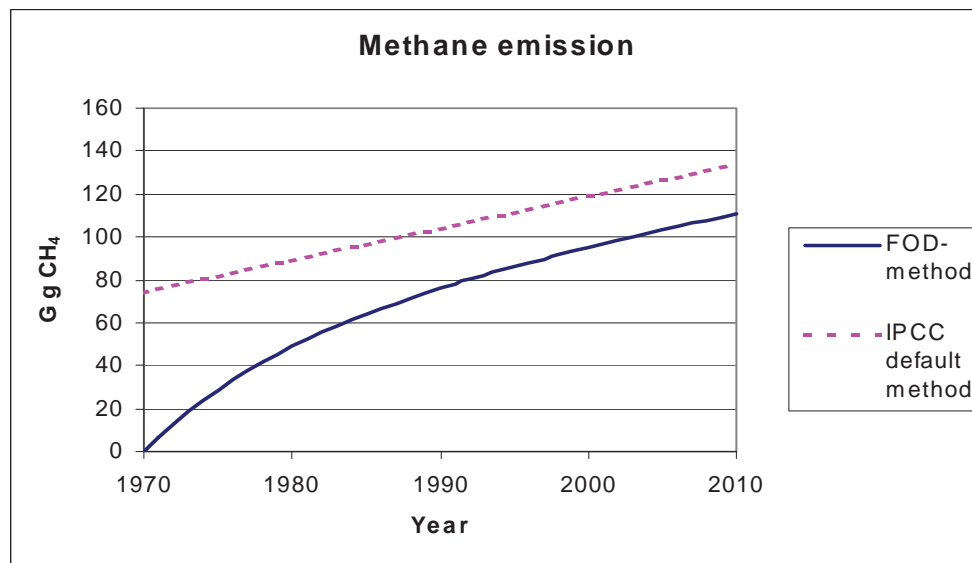
Figure 2 Emissions with default and FOD models with continuous growth in SW disposal
