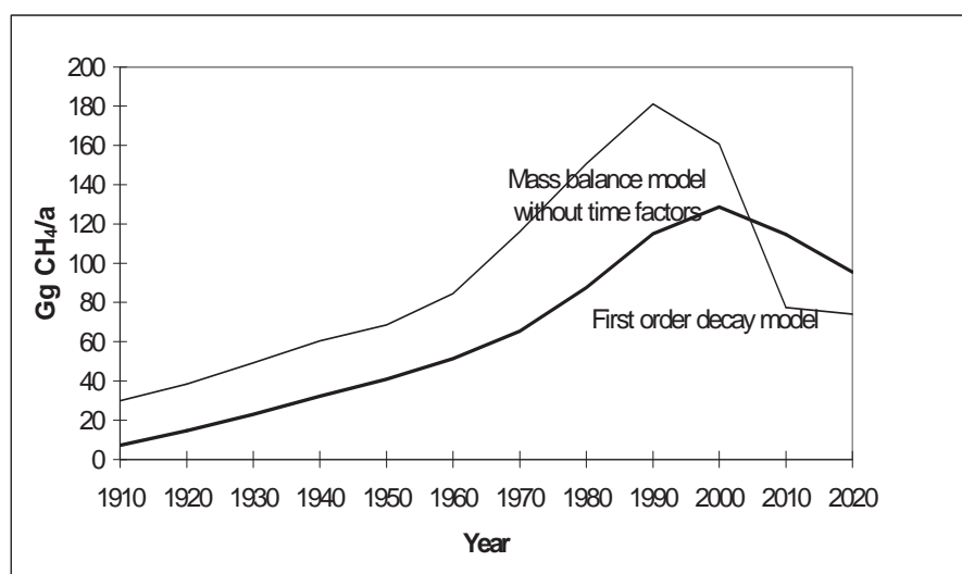
Figure 1 Emissions with the default (A) and FOD (B) models with growth and then reduction in SW disposal
