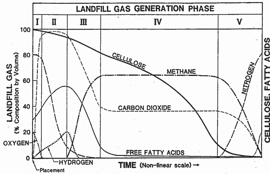
Figure 3 Composition of landfill gas in different phases of the degradation process
